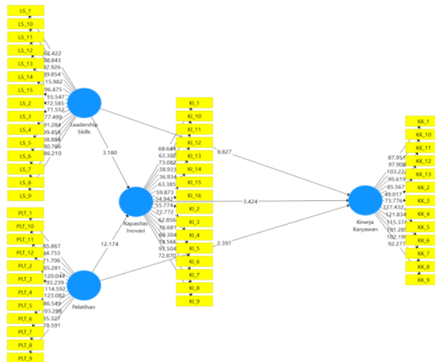
Figure 2 PLS Algorithm
